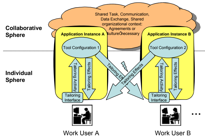
Figure 3. Collaboration in "Shared Context" scenarios
